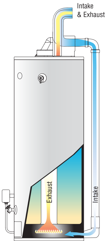
Direct vent gas water heater
